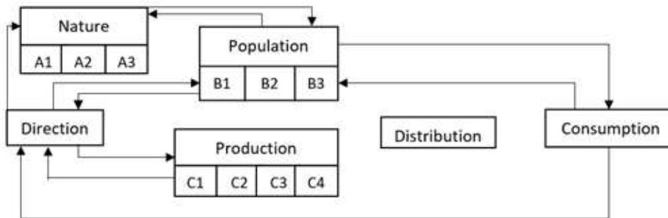
Fig. 1. Socio-economic status of territorial systems development control chart.
