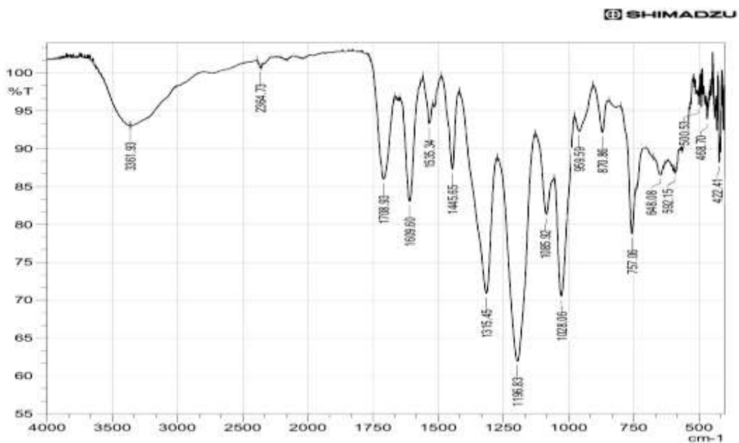
IR spectrum of polyphenols in the dome of the plant Pinus sylvestris L.
