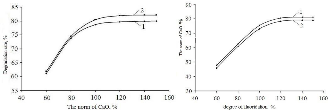
Figure.1. Effects of calcium carbonate (1) and UCFC (2) levels on fluorination
