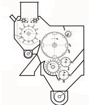
Figure 1. BCh-2M sawdust cleaner
