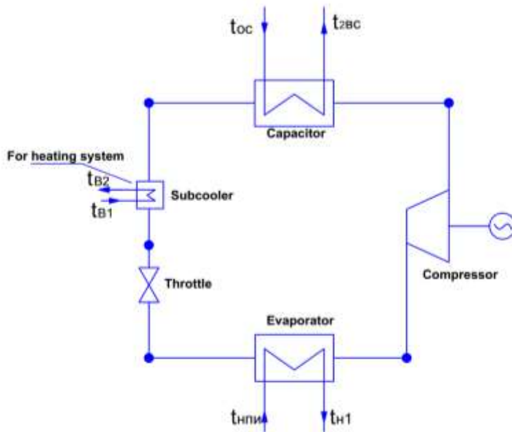
Figure 1. - Schematic diagram of a vapor compression heat pump installation with a pre-cooler.
